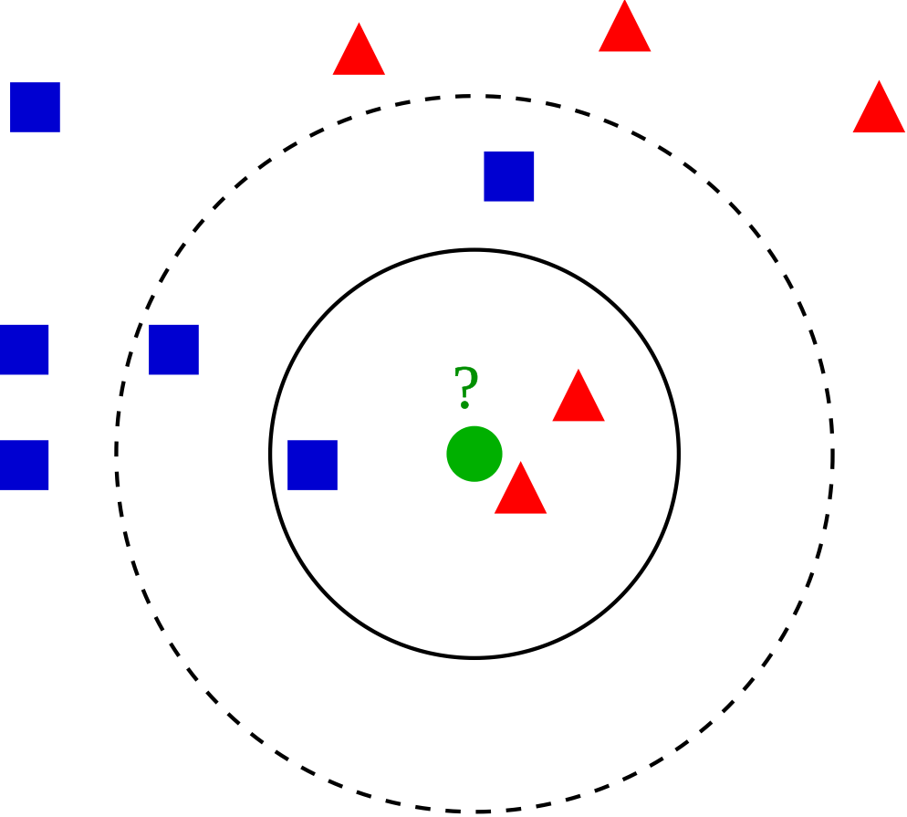
K-NN Classification
