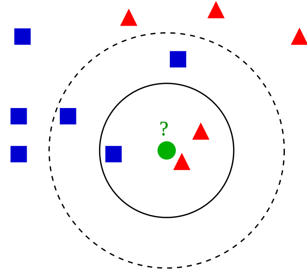
K-NN Classification
