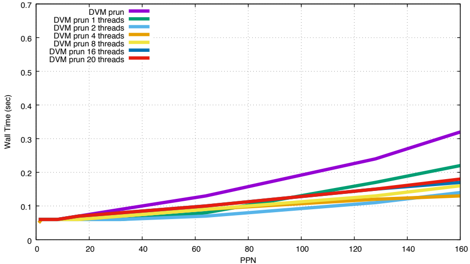
PPN Scaling, 1 node x 2 socket x 10 cores x 8 hwthreads
