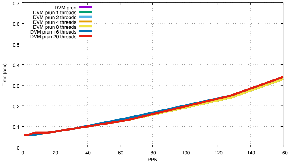
PPN Scaling, 1 node x 2 socket x 10 cores x 8 hwthreads
