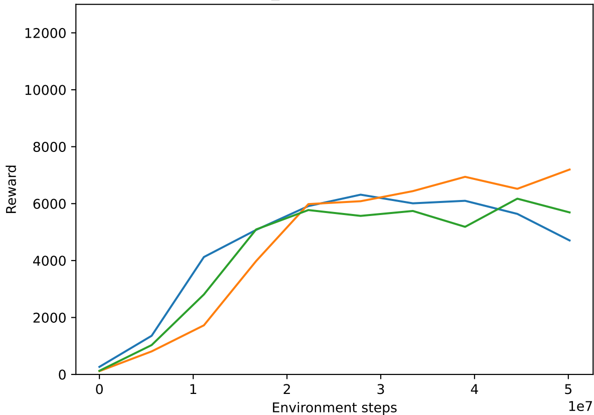
humanoid_scaled (3 random seeds)
