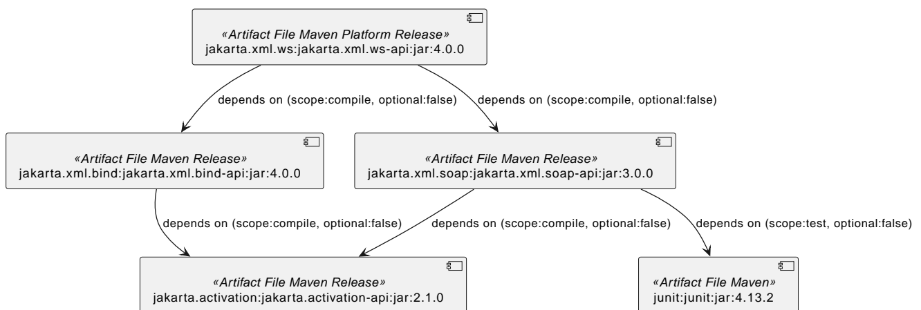
Figure 62. Jakarta XML Web Services API 4.0.0 actual
