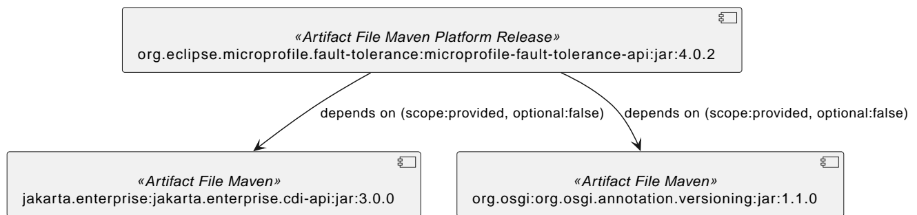
Figure 84. MicroProfile Fault Tolerance API 4.0.2 actual
