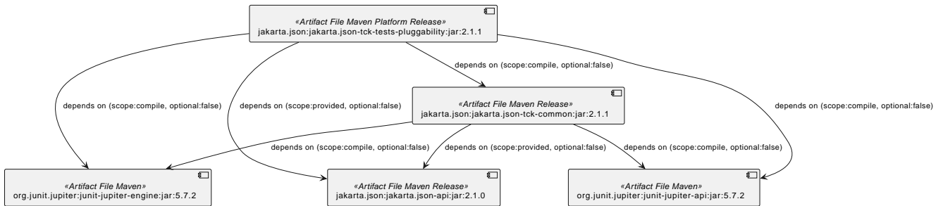
Figure 39. Jakarta JSON TCK Tests Pluggability 2.1.1 actual
