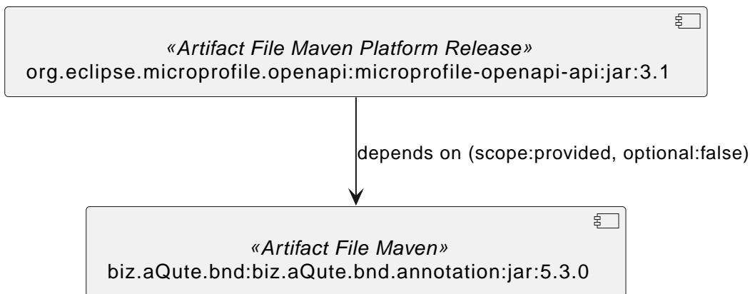
Figure 96. MicroProfile OpenAPI API 3.1 actual
