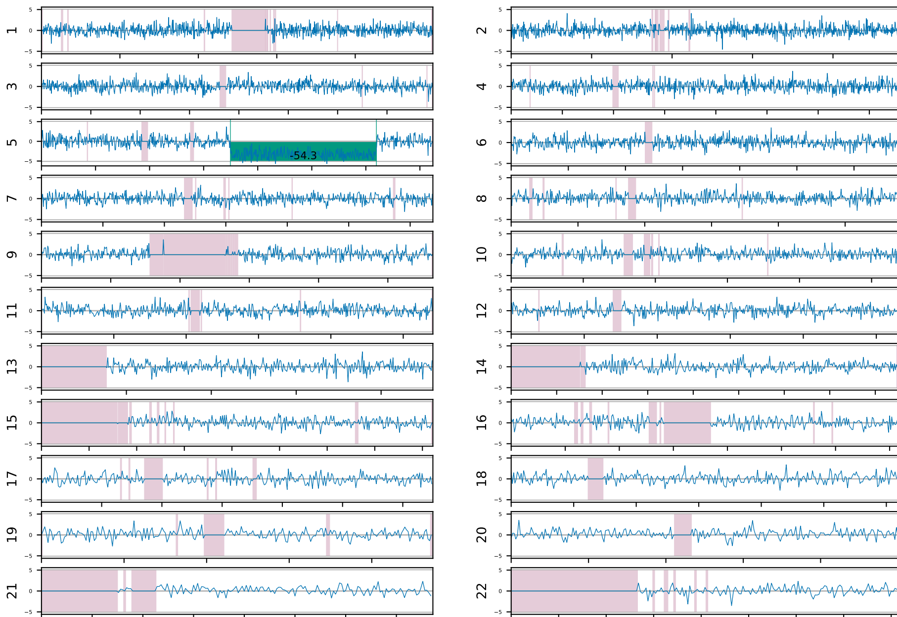
Z-score versus chromosomal position - Sample NA-349_out
