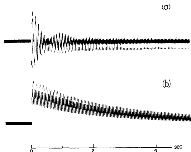
FIG. 4. As Fig. 2, but with pulse rate of 22 per second. In these records the " 180^\circ pulses" were intentionally made too weak, and gave actually about 171^\circ flips. The error is cumulative in record a , but not in record b , which was made with 90^\circ phase shift of the first pulse.
