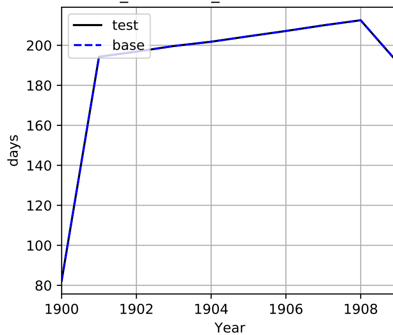
SITE_DAYSINCE_DROUGHTLEAFOFF
