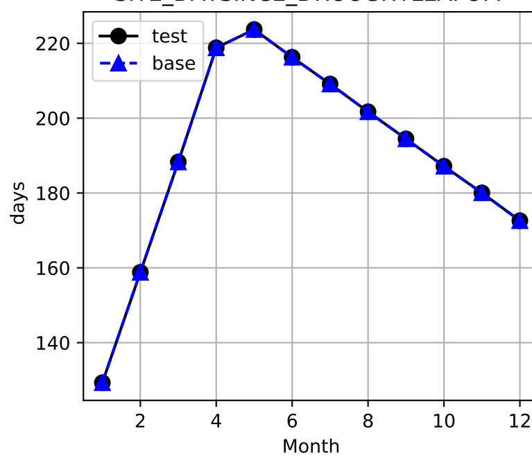
SITE_DAYSINCE_DROUGHTLEAFOFF
