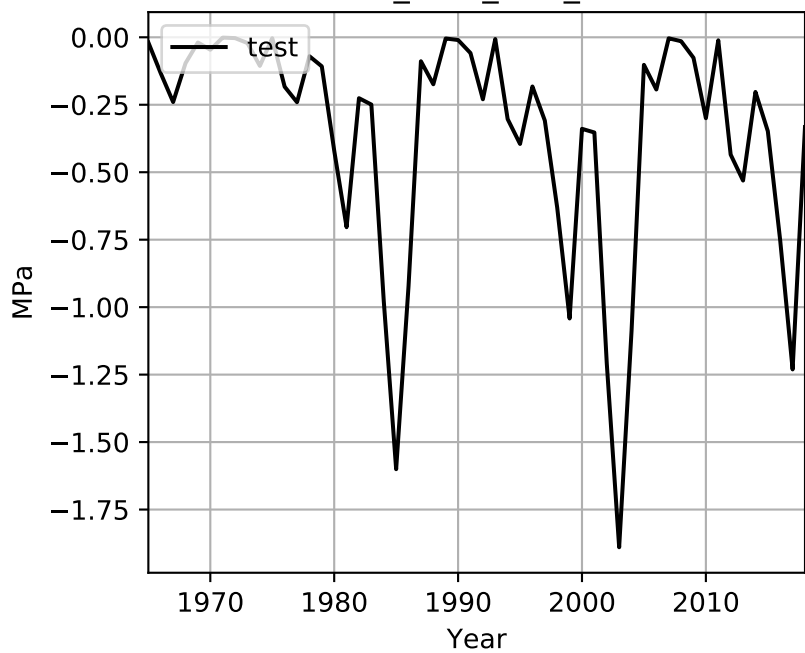
FATES_AWP_COL_SCPF
