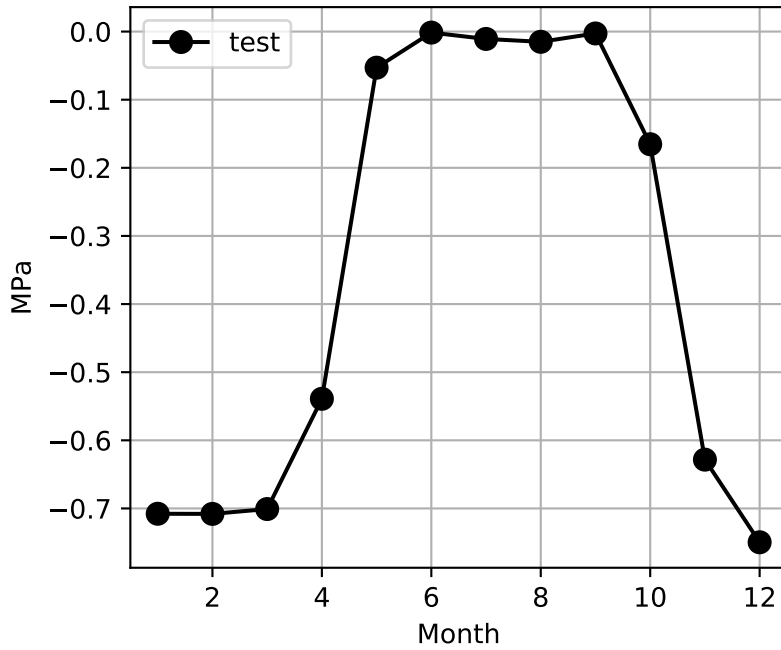
FATES_AWP_COL_SCPF
