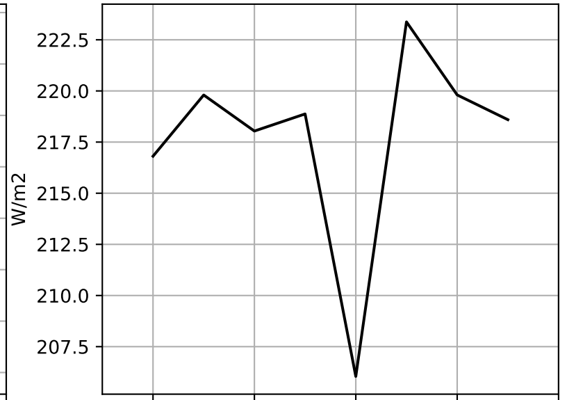
FSDS
