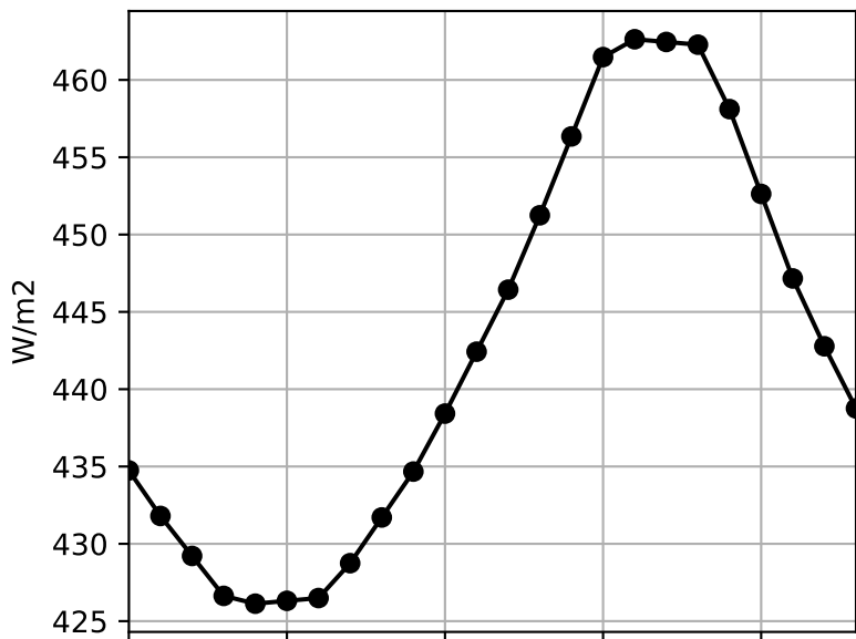
FLDS
